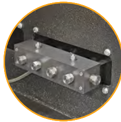
Multi-Port Manifold Outlet, allows multiple hose assemblies to be tested at the same time.
